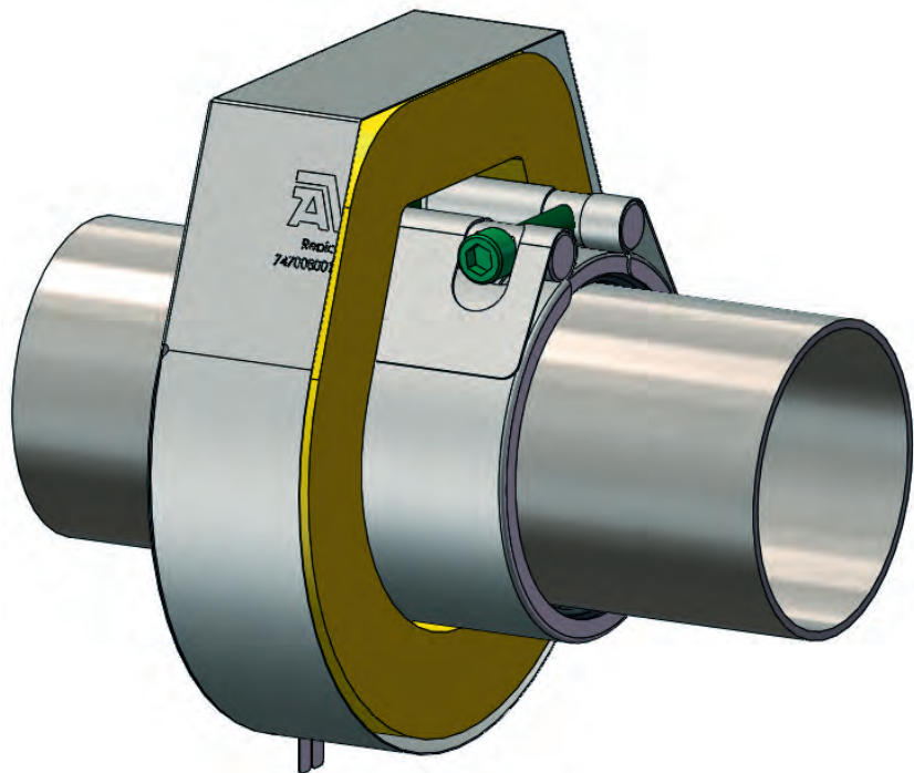
AVK Repico® - Fire resistant cover (FRC) Stainless steel 316, EPDM rubber
